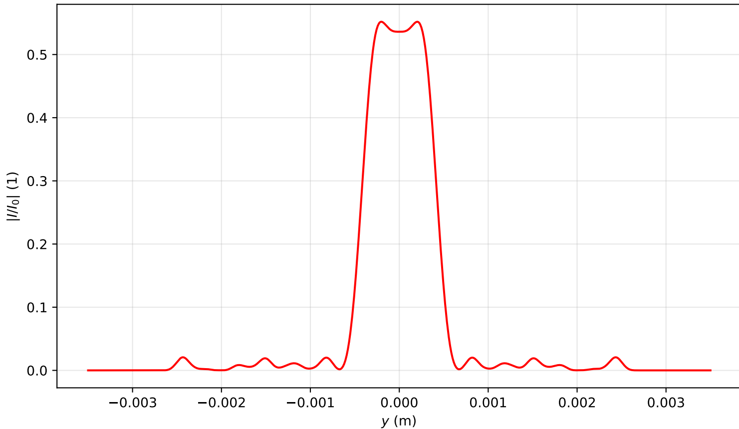
Intensity profile I(x=0, y, z=3.344)/I_0 , \text{Pin}=3.0\text{Pcr} , artificial time
